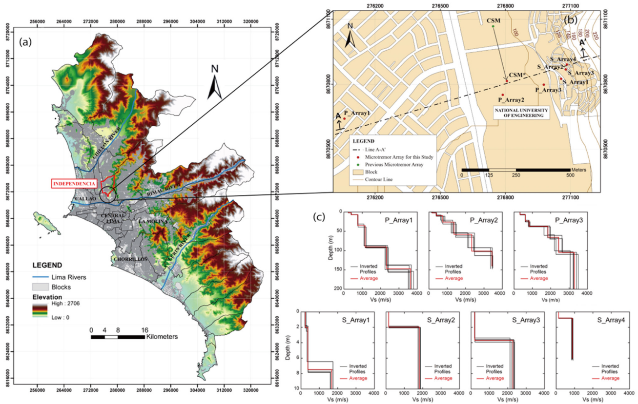
Fig. 1. (a) Elevation map of the city of Lima and Independencia district (red line). (b) Location of the microtremor arrays. (c) Calculated shear-wave velocity profiles along line A-A' [2].
