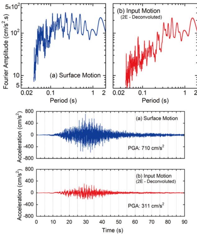
Fig. 3. Fourier spectra and time-histories for (a) surface motion and (b) deconvoluted input motion.
