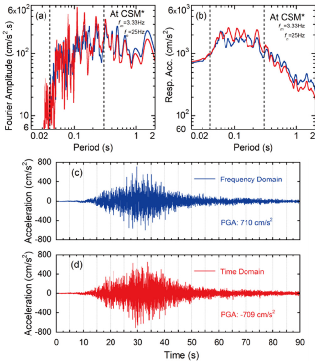
Fig. 5. (a) Fourier spectra, (b) acceleration response spectra, and (c) waveforms for the frequency domain and (d) the time domain (FEM): results at CSM* ( f_m = 3.33 Hz and f_n = 25 Hz).
