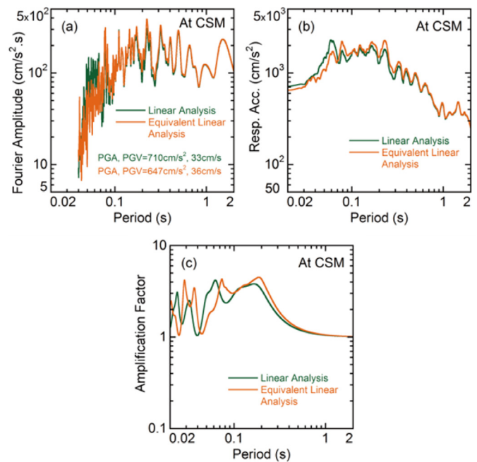
Fig. 4. (a) Fourier spectra, (b) acceleration response spectra and (c) transfer functions for linear and equivalent linear cases.
